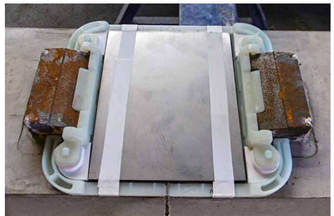
Figure 5: Intermediate pad with sensor at rail seat
