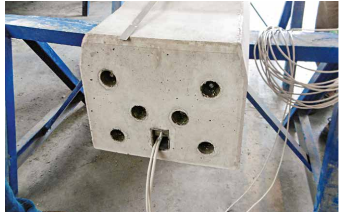
Figure 3: Sleeper cross section with IMS embedded into the sleeper body
